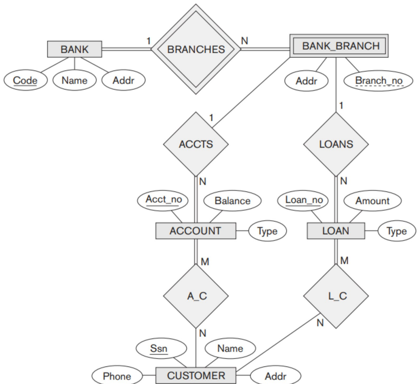
Figure : An ER diagram for a BANK database.
